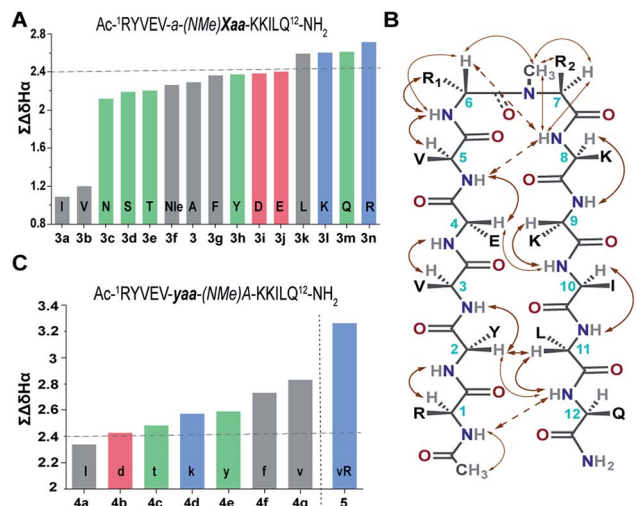
Fig. 4 (A) \Sigma CSD of the primary library with L-amino acid substitutions (Xaa) at the i +2 site. (B) The characteristic NOEs, where the thick arrows denote strong (1.8–2.1 Å), the thin arrows denote medium (2.2–2.5 Å) and the broken arrows denote weak (>2.6 Å) NOEs. (C) \Sigma CSD of the secondary library with i +1 substitutions (yaa) along with 5 derived from the combination of 4g and 3n. All the NMR measurements were done in acetate buffer (pH 3.8) at 25 °C.
