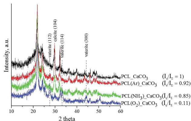
Fig. 4 XRD spectra of PCL/CaCO 3 scaffolds before and after plasma treatment. The ratio of the integrated intensity of the calcite phase ( I_c ) to the total integrated intensity ( I_t ) represents the relative proportion of the calcite phase in the deposited coatings.
