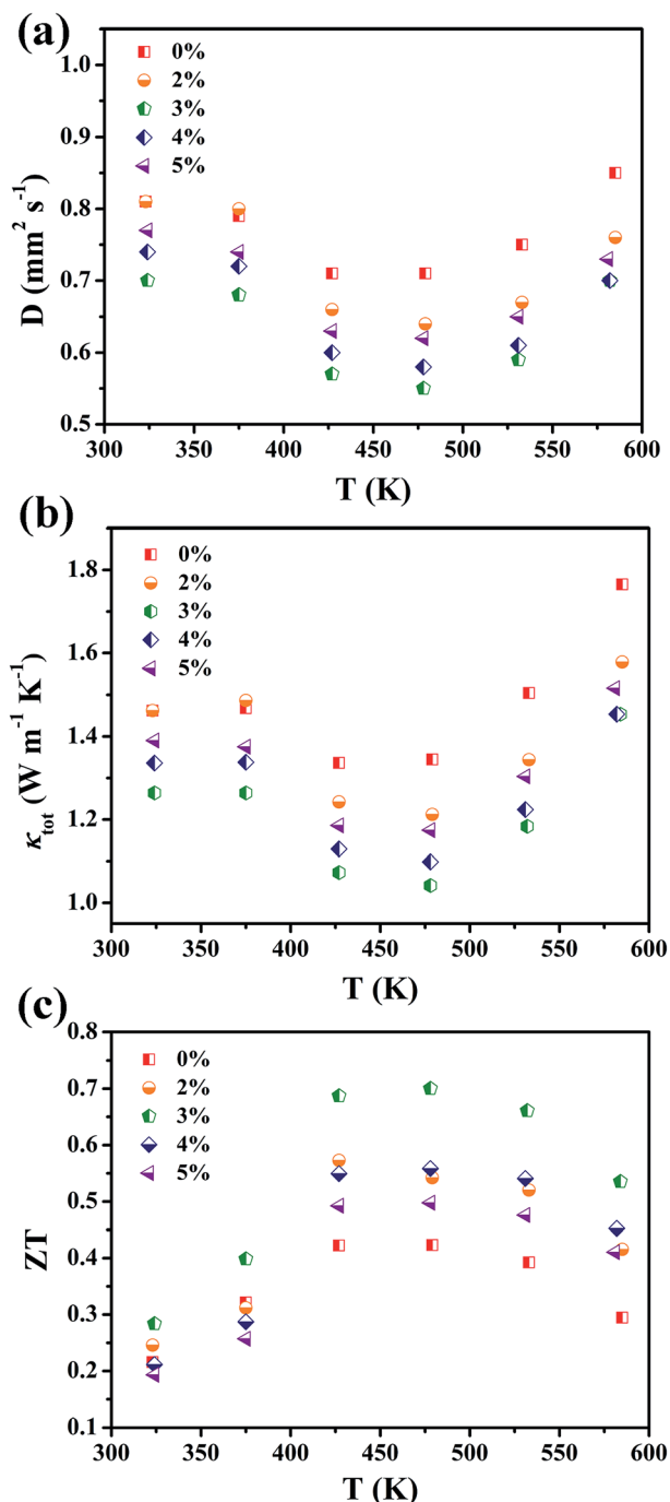
Fig. 5 Temperature-dependent (a) diffusivity coefficient; (b) thermal conductivity and (c) ZT values for \text{Mg}_{1-x}\text{Zn}_x\text{Ag}_{0.9}\text{Sb}_{0.95} ( x = 0-5\% ), respectively.
