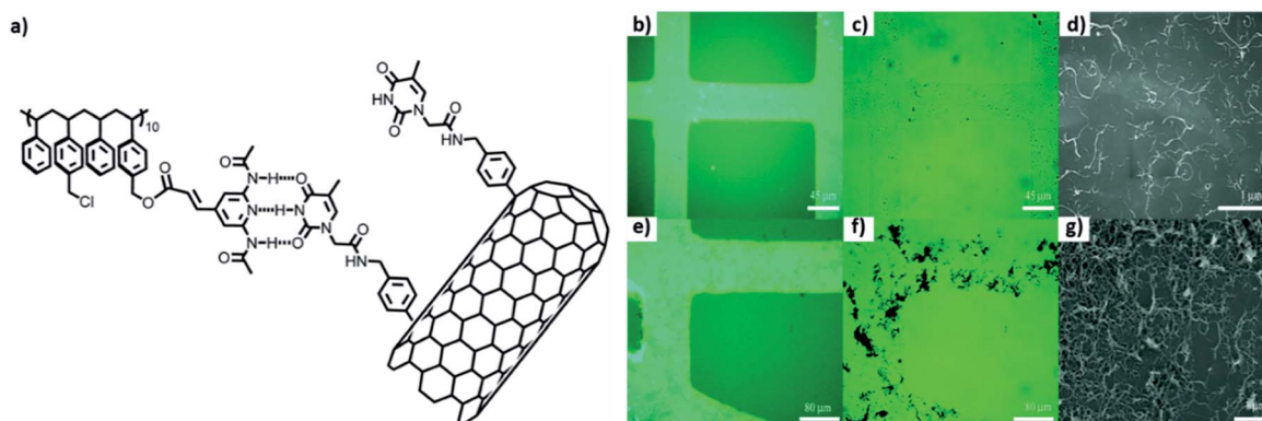
Fig. 22 (a) Chemical structure of PS1, thymine-MWCNTs; images of patterned surface by (b) and (e) fluorescence, (c) and (f) optical and (d) and (g) scanning electron microscopy, after deposition of a dispersion of Thymine-MWCNTs in DMF (b-d) and CHCl 3 (e-g). (Reproduced with permission from ref. 115 © 2012 American Chemical Society).
