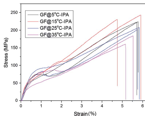
Fig. 7 Stress–strain curves of GOFs obtained in isopropanol at different temperatures.
