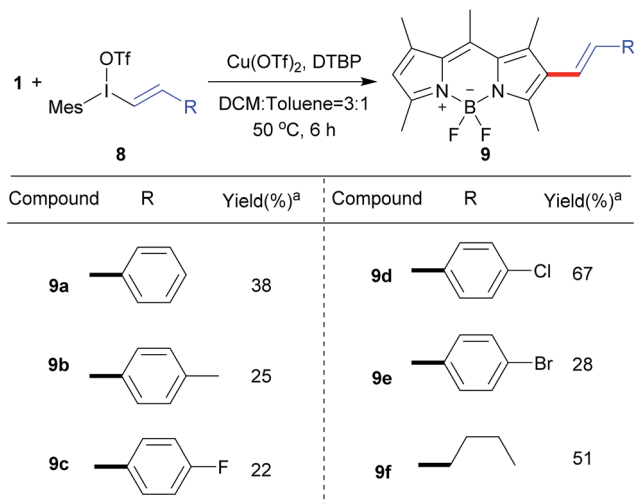
Scheme 5 Scope of the direct C–H vinylation of BODIPY 1 with different vinyltriflate salts. a Isolated yield.
