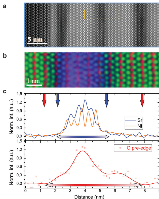
Fig. 4 HR-STEM investigation for the \text{La}_{0.7}\text{Sr}_{1.3}\text{NiO}_4/\text{La}_2\text{CuO}_4 interface. (a) HAADF image of a LSNO/LCO superlattice structure ( N = 9 ). (b) Spatial elemental distribution, extracted from the EELS spectrum image across a \text{La}_{0.7}\text{Sr}_{1.3}\text{NiO}_4 region and neighboring LCO areas (the analyzed region is highlighted by the orange square in panel (a)). The color code is as follows: La-green, Cu-red, Ni-orange, Sr-blue. (c) EDX signal for Sr (blue) and Ni (orange) (top panel), together with the simultaneously acquired O-K edge prepeak profile as obtained by a EELS linescan (red line, bottom panel). The blue and red arrows indicate the upper limits for the Sr and holes distributions, respectively.
