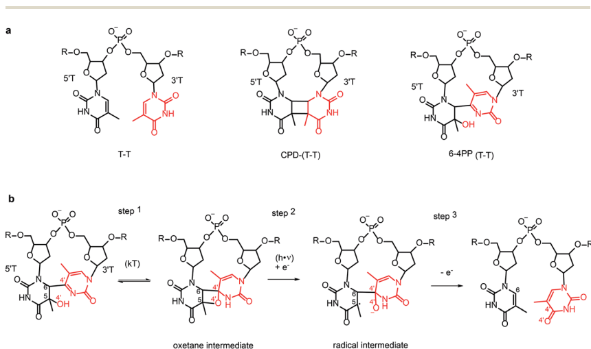
Scheme 1 (a) Chemical structure of the T–T dinucleotide and its CPD and 6–4 PP photolesions; (b) sequence of steps involved in the hypothesized repair of 6–4 PP photolesions by 6–4 photolyase via formation and photoreactivation of the oxetane intermediate. The atoms of the 3' base (3'T) are shown in red.
