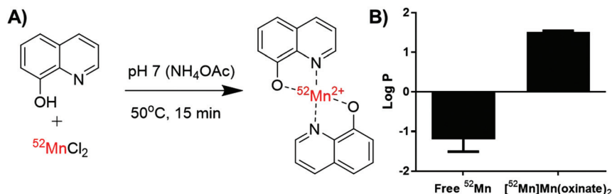
Fig. 2 (A) Radiochemical scheme for the synthesis of ^{52}\text{Mn} ][Mn(oxinate) _2 , and (B) chart showing the \log P values of unchelated ^{52}\text{Mn} and ^{52}\text{Mn} ][Mn(oxinate) _2 in water/octanol. Error bars represent standard deviation ( n = 2 ).
