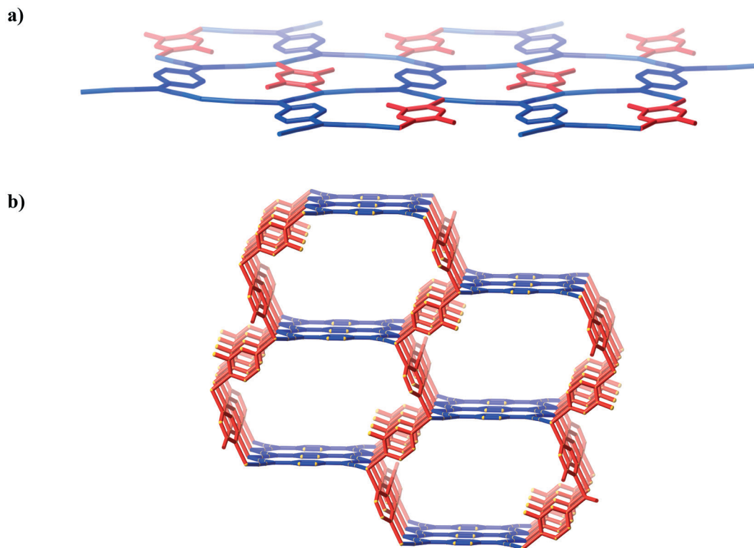
Fig. 10 a) The 2D sheet structure of [\text{Cu}_{12}(\text{TCNQ})(\text{Me}_2\text{pyz})_2] (61) (TCNQ ^{2-} represented in blue; Me _2 pyz represented in red). b) The 3D coordination polymer [\text{Cu}_{12}(\text{TCNQ})(2\text{-aminopyrazine})_2] (62); for clarity, only one orientation of the disordered 2-aminopyrazine ligands is shown (TCNQ ^{2-} represented in blue; 2-aminopyrazine represented in red).
