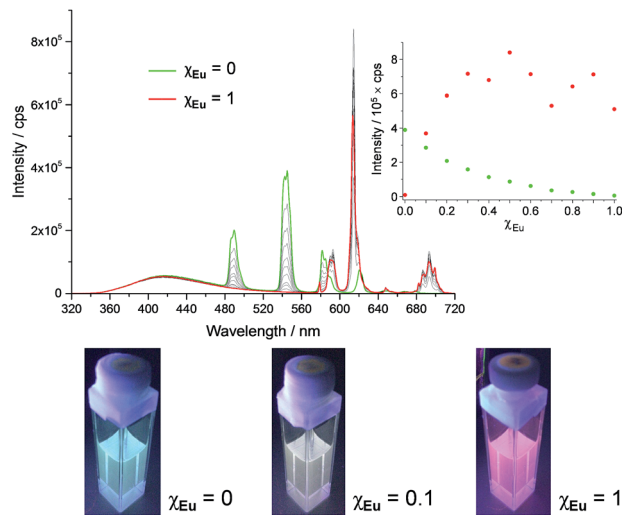
Fig. 4 Fluorescence emission spectra of \mathbf{tdt}[\text{Eu}(\text{EDTA})]_x[\text{Tb}(\text{EDTA})]_{3-x} assemblies in methanol as a function of \chi_{\text{Eu}} and corresponding pictures for \chi_{\text{Eu}} = 0, 0.1 and 1 ; inset: experimental binding isotherms for the \text{Eu}(\text{III}) - (●) and \text{Tb}(\text{III}) -centred (●) emission; [\mathbf{tdt}] = 25 \mu\text{M} and \lambda_{\text{ex}} = 270 \text{ nm} .
