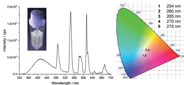
Fig. 5 Fluorescence emission spectra ( \lambda_{\text{ex}} = 270 \text{ nm} ) and CIE-1931 chromaticity diagram for \mathbf{tdt}[\text{Eu}(\text{EDTA})]_{0.3}[\text{Tb}(\text{EDTA})]_{2.7} in methanol as a function of the excitation wavelength; [\mathbf{tdt}] = 25 \mu\text{M} and \chi_{\text{Eu}} = 0.1 . Inset shows the corresponding photograph obtained with \lambda_{\text{ex}} = 270 \text{ nm} .
