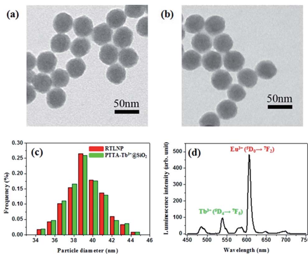
Fig. 3 TEM images of PTTA-Tb ^{3+} -encapsulated silica particles (a) and RTLNP particles (b). (c) Particle size distribution histograms of the two kinds of nanoparticles. (d) Time-gated emission spectrum of the RTLNP ( 50 \mu\text{g ml}^{-1} ) in 1 : 4 ethanol–0.05 M PBS buffer of pH 7.4 ( \lambda_{\text{ex}} = 330 nm).
