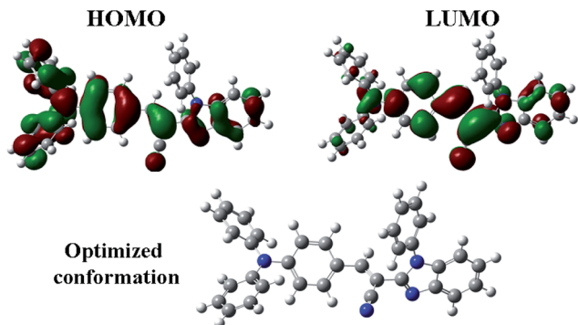
Fig. 2 Electron density distributions in the HOMO and LUMO states of TBM calculated by DFT in Gaussian 09 at the B3LYP/6-31G(d) level.
