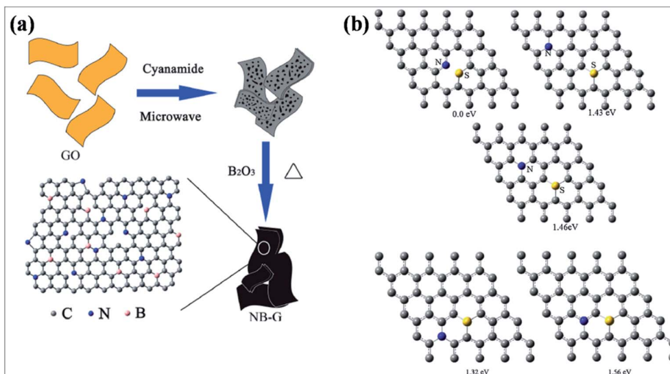
Fig. 27 (a) Fabrication of the NB-G framework from GO. Reproduced with permission. 287 © 2013 Royal Society of Chemistry. (b) Optimized unit cells for 5 \times 5 sulfur and nitrogen dual-doped graphene. Reproduced with permission. 285 © 2014 Elsevier.
