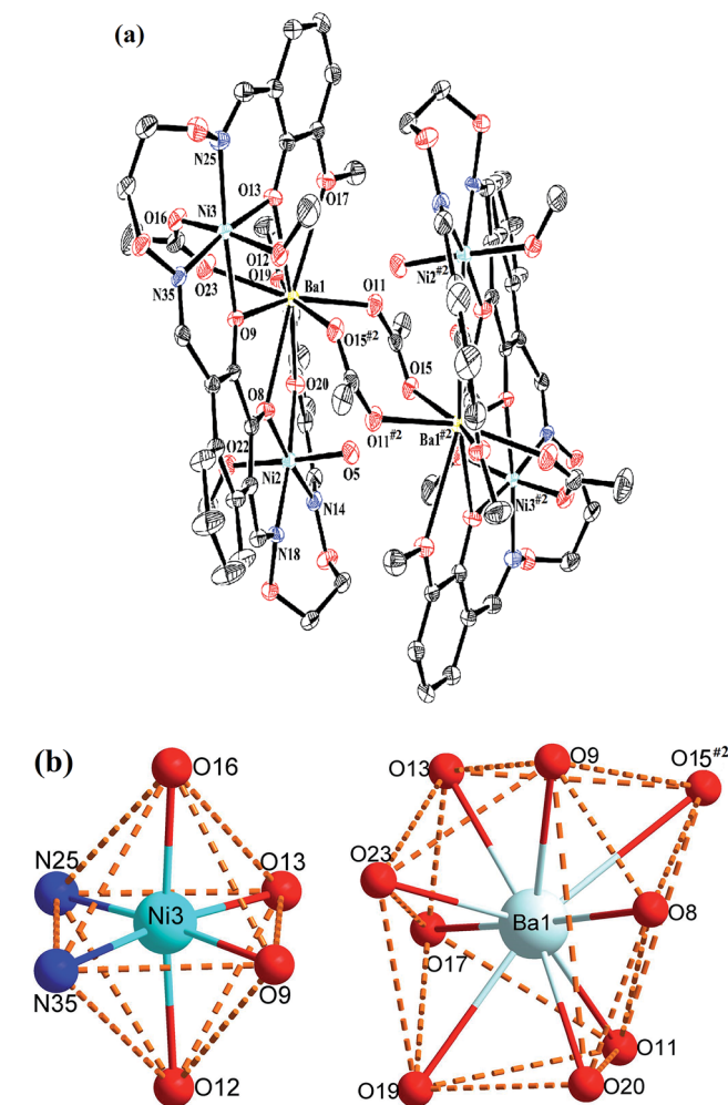
Fig. 6 (a) View of the molecular structure of complex 3 (hydrogen atoms are omitted for clarity, and thermal ellipsoids are drawn at the 30% probability level). (b) Coordination polyhedra for Ni(II) and Ba(II) atoms of complex 3.
