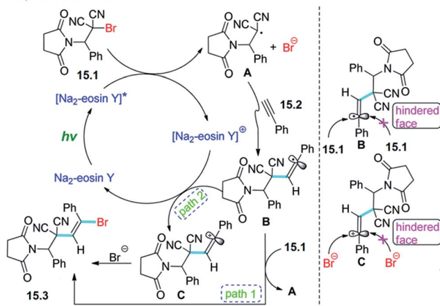
Scheme 15 Difunctionalization of alkynes with alkyl bromides.
