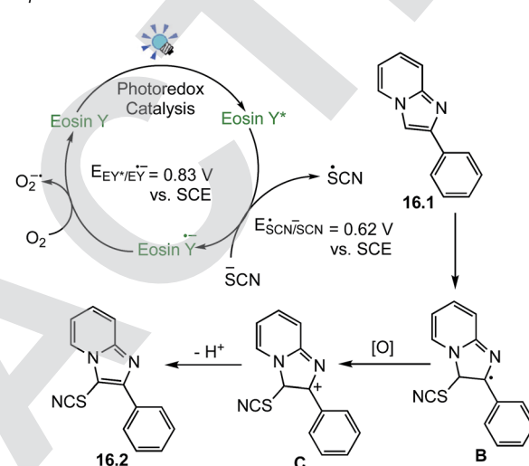
Scheme 16 Thiocyanation of imidazoheterocycles.
