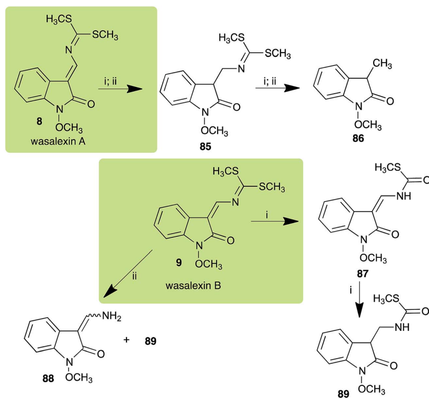
Scheme 3 Detoxification of the cruciferous phytoalexins wasalexin A ( 8 ) and wasalexin B ( 9 ) by plant fungal pathogens: (i) Leptosphaeria maculans (canola virulent isolates); (ii) L. maculans (brown mustard virulent isolates).
