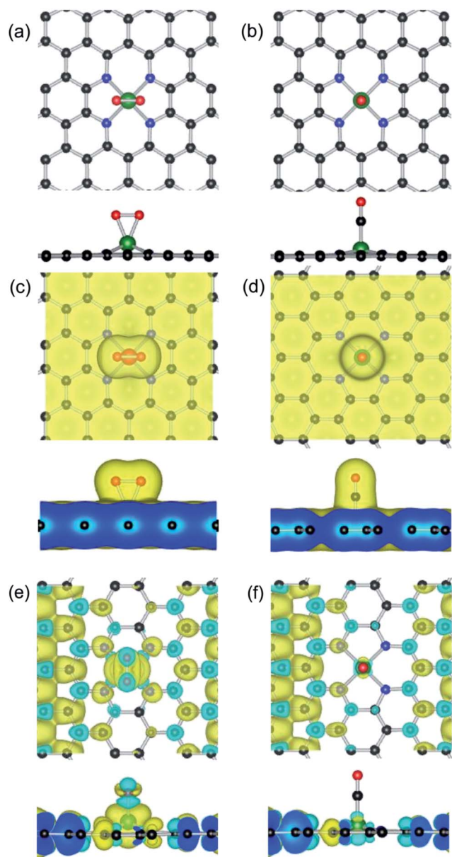
Fig. 3 Top and side views of the (a and b) geometric structures, (c and d) charge distribution and (e and f) spin charge density plots for \text{O}_2 and CO adsorbed on the Fe–GN4 surface. Black, blue, red and green balls represent the C, N, O and Fe atoms, respectively.
