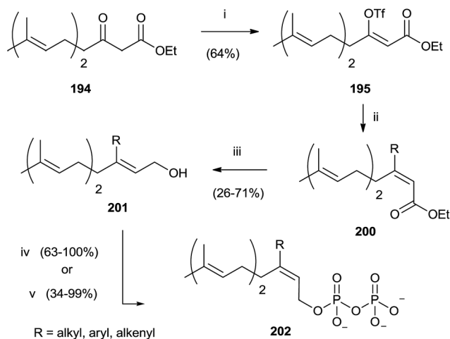
Scheme 35 Reagents and conditions: (i) (\text{Me}_3\text{Si})_2\text{NK} , THF, \text{PhN(SO}_2\text{-CF}_3)_2 . (ii) \text{RMgX} , CuCN, ether. (iii) DIBALH, toluene. (iv) a: NBS, \text{CH}_2\text{Cl}_2 , \text{Me}_2\text{S} ; b: (\text{Bu}_4\text{N})_3\text{HP}_2\text{O}_7 , \text{CH}_3\text{CN} .
