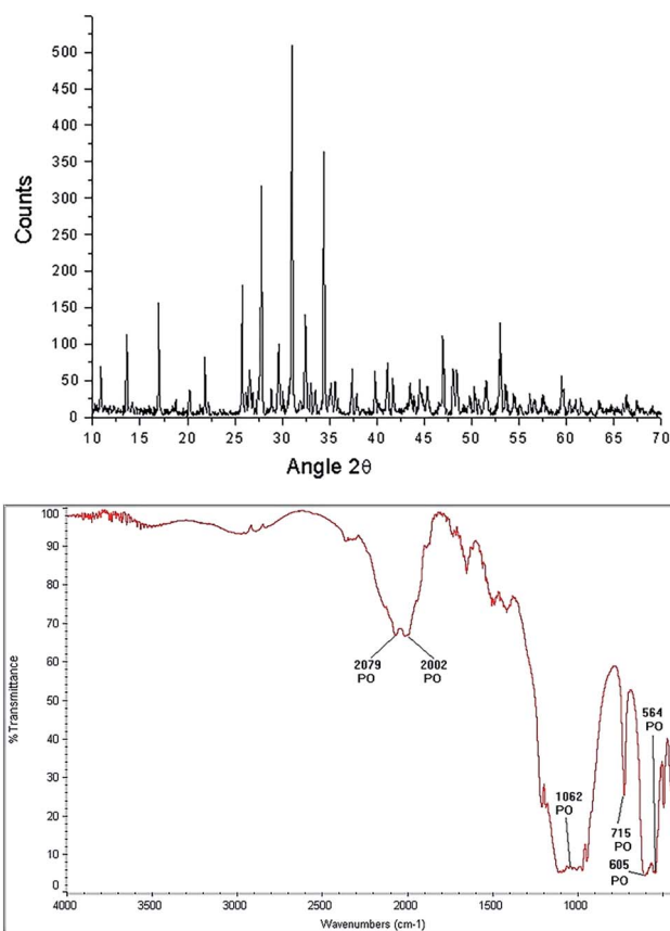
Fig. 7 Characterization of the \beta -TCP phase: diffractogram (up) and FTIR spectrogram (bottom).
