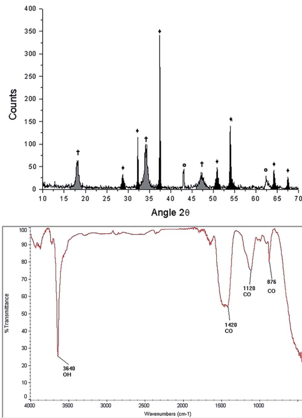
Fig. 5 Characterization of the starfish Mellita eduardobarrosi sp. nov. after the thermal treatment: diffractogram (up) showing the phases: †[Ca(OH) 2 ], ♦[CaO], °[MgO], and FTIR spectrogram (bottom).
