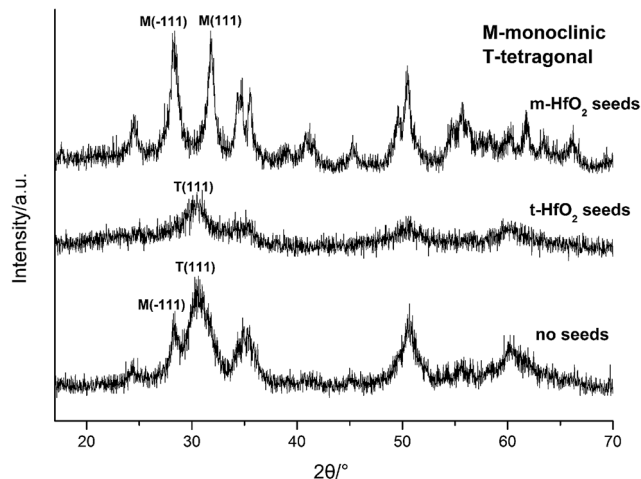
Fig. 9 XRD spectra of \text{HfO}_2 NPs prepared with different seeds.
