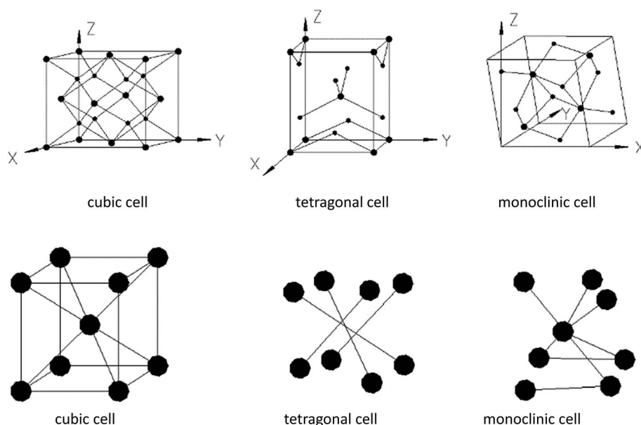
Fig. 10 Structures of different \text{HfO}_2 crystal cells.
