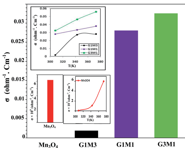
Fig. 12 Conductivity results of \text{Mn}_3\text{O}_4 , G3M1, G1M1 and G1M3 samples measured at room temperature and at 373 K. Inset is the \sigma vs. T for exploring the effect of increasing temperature on the conductivity.
