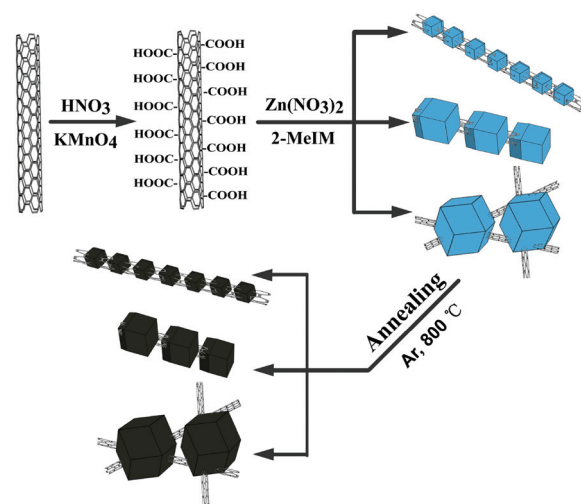
Fig. 1 Synthetic scheme for the fabrication of MWCNT/NPC-S/M/L.
