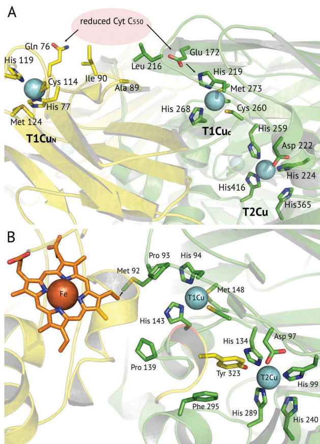
Fig. 6 Proposed electron transfer routes between the redox centres of 3-domain CuNiRs. In (A) HdNiR the external electron donor partner protein cyt. c 550 is proposed to bind to a hydrophobic patch spanning the N-terminal (near Ala89, Ile90) and cupredoxin domains (near Leu216), where it is positioned for electron transfer to both the T1Cu N and T1Cu C sites (indicated by arrows). 74 In (B) RpNiR , the proposed internal electron transfer route is from the haem (CBC atom) to Met92 and to the T1Cu site. 75 Interface and T2Cu water molecules have been omitted from the figures for clarity.
