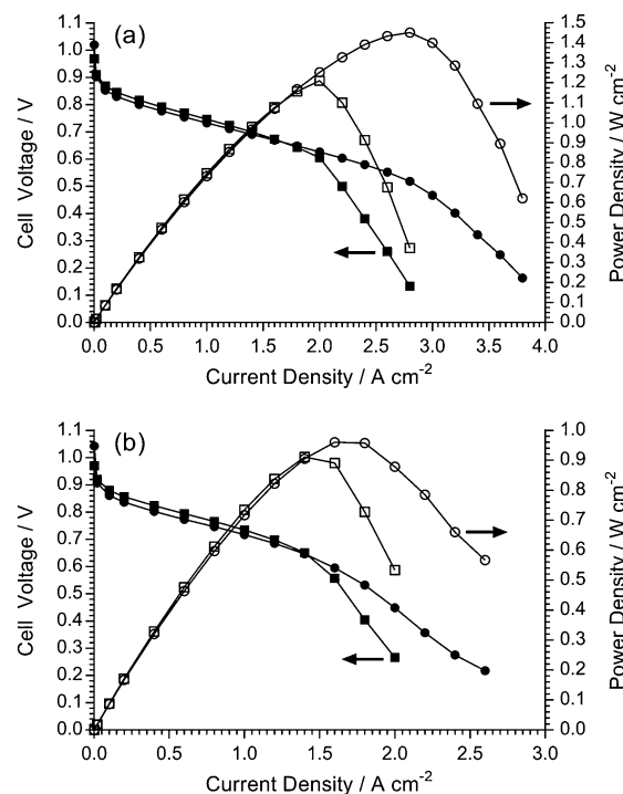
Fig. 12 The \text{H}_2/\text{O}_2 AEMFC performances of the LDPE-AEM (100 kGy) (●, ○) and ETFE (30 kGy) (■, □) at (a) 80 \text{ }^\circ\text{C} and (b) 60 \text{ }^\circ\text{C} : PtRu/C (50% wt Pt and 25% wt Ru) anodes and Pt/C (40% wt) cathodes (all 0.4 \text{ mg}_{\text{Pt}} \text{ cm}^{-2} loadings). The 1.0 SLPM gas supplies contained 10 ppm \text{CO}_2 contamination and were not pressurised: relative humidity (RH) = 68% for the 60 \text{ }^\circ\text{C} tests and RH = 100% for the 80 \text{ }^\circ\text{C} tests (these humidity levels were optimised for maximum performance at each cell temperature).
