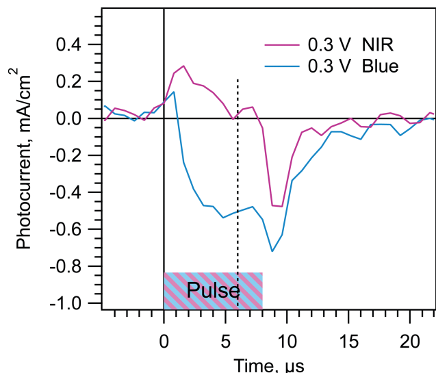
Fig. 5 Effect of blue vs. NIR (735 nm) pulses at V_d and t_d where the photocurrents from regions I and III vs. region II are balanced for the NIR pulse. The peaks at 1 \mu s and 9 \mu s are from the switching of the LED. Data from a m-TiO 2 /MAPI cell with t_d = 2 ms and V_d = 0.3 V.
