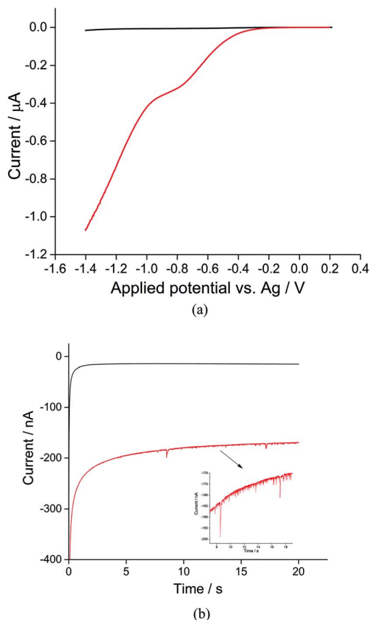
Fig. 1 (a) Linear sweep voltammograms and (b) chronoamperograms at -1.4\text{ V} vs. silver pseudo-reference electrode of the toluene emulsion taken in the nitrogen-degassed (black) and oxygenated (red) states using a microwire electrode. If cyclic voltammetry is recorded in (a) the reverse scan is essentially superimposed on the forward scan.
