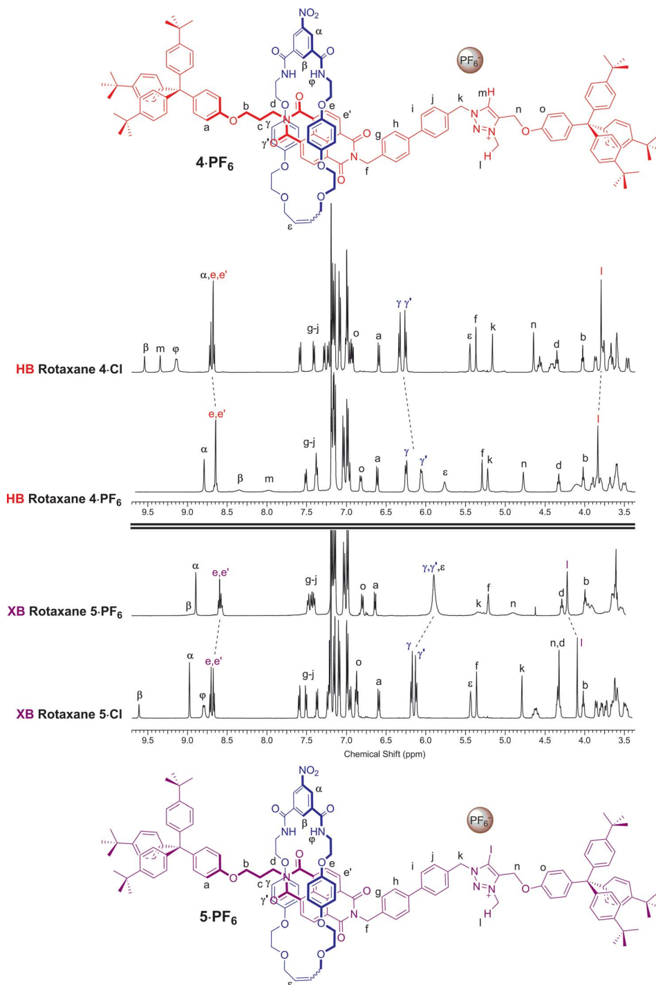
Fig. 3 Comparison of the truncated ^1\text{H} NMR spectra ( \text{CDCl}_3 , 298 K, 400 MHz) of [2]rotaxanes 4·Cl, 5·Cl, 4·PF 6 and 5·PF 6 with their predicted co-conformations in the presence of PF 6 - .
