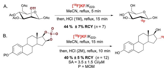
Scheme 1 (A.) Radiosynthesis of 2- [^{18}\text{F}] fluoro-2-deoxy-D-glucose ( [^{18}\text{F}] FDG). (B.) Radiosynthesis of 16- \alpha - [^{18}\text{F}] fluoroestradiol ( [^{18}\text{F}] FES). SA = specific activity. MOM = methoxymethyl.
