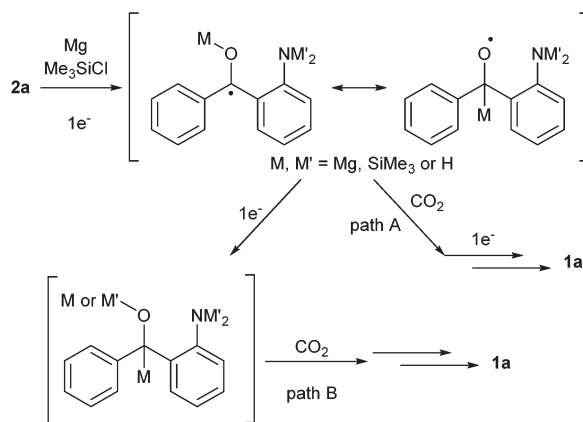
Scheme 4 Plausible paths for the synthesis of oxindoles 1a via reductive coupling of 2a and CO 2 .
