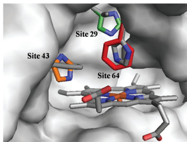
Fig. 1 Structures of the heme pocket of sperm whale myoglobin (gray). And the residues mutated in our studies are also shown: His-29 (green), His-43 (orange), and Phe-64 (red). All N atoms are marked in blue. The PDB code for wild-type Mb is 1JP6. Structures of mutants were reproduced by PyMol.
