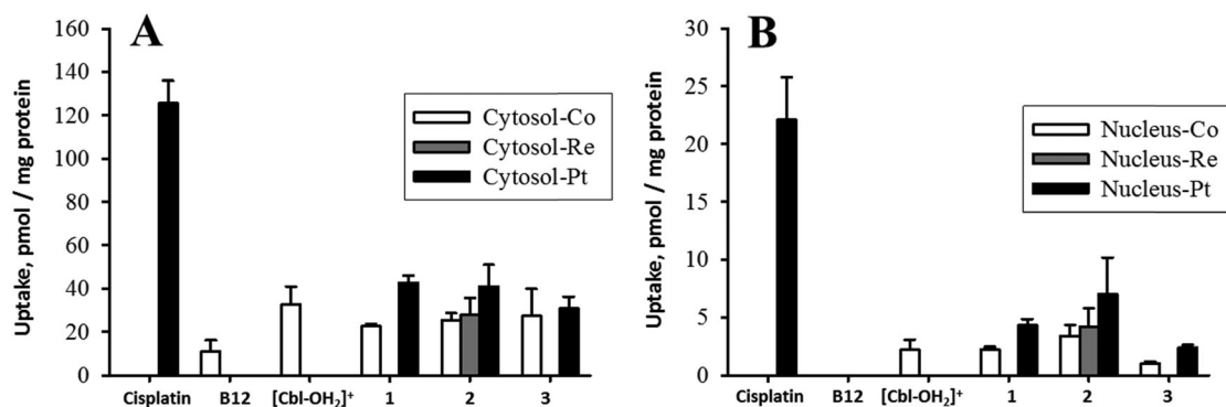
Fig. 5 Uptake in K562 cellular cytosol (A) and nucleus (B) of [(\text{Co})-\text{CN}-(\text{cis}-\text{PtCl}(\text{NH}_3)_2)]^+ ( 1 ), [(\text{Re})-(\text{Co})-\text{CN}-(\text{cis}-\text{PtCl}(\text{NH}_3)_2)]^+ ( 2 ), and [(\text{Co})-\text{CN}-(\text{trans}-\text{Pt}(\text{Cyt})(\text{NH}_3)_2)]^{2+} ( 3 ). Cisplatin, B12, [\text{Cbl}-\text{OH}_2]^+ were included as control samples.
