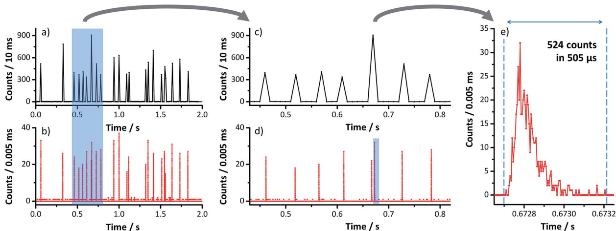
Fig. 1 Representative ICP-MS signal (monitoring m/z ^{197}\text{Au} ) due to 30 nm AuNPs ( C_{\text{NP}} = 2.5 \times 10^5 NP mL ^{-1} ) acquired simultaneously for 2 s with (a) 10 ms dwell time (vendor software), and (b) 5 \mu\text{s} dwell time (home-built DAQ). First zoom level shows several particle events in (c) and (d) for 500 ms (of highlighted section in a and b). Second zoom level (e) shows the temporal profile of a single particle's ion cloud identified with the home-built DAQ in (d).
