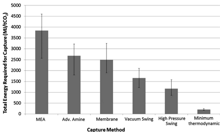
Fig. 1 Comparison of calculated energy costs of different CO 2 capture methods: MEA, 16 advanced amine, 17 membrane, 18 vacuum swing. 19 High pressure swing was calculated from the preliminary process model [see main text] and was found to be in agreement with literature values. 20 Minimum thermodynamic separation costs were calculated from entropy of de-mixing.
