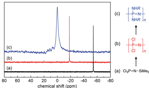
Fig. 4 Sample ^{31}\text{P}\{^1\text{H}\} NMR spectra of the monomer trichlorophosphoranimine \text{Cl}_3\text{PNSiMe}_3 (a), polydichlorophosphazene [\text{NPCI}_2]_n (b) and a macrosubstituted poly(organo)phosphazene [\text{NP}(\text{NHR})_2]_n (c) demonstrating the simple tracking of the reaction progression. Adapted from H. Henke et al. , J. Polym. Sci., Part A: Polym. Chem. , 2013, 51 , 4467. Copyright 2013 Wiley Periodicals, Inc. 12
