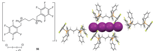
Fig. 30 Molecular structure and representative part of the crystal structure of 56 showing the unstable I_4^{2-} anion stabilized by CH-anion and anion- \pi interactions.
