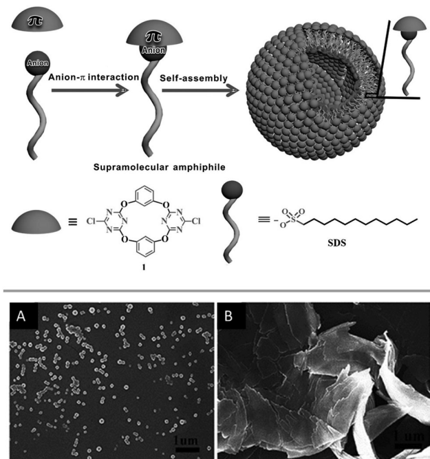
Fig. 34 Schematic representation of the anion- \pi induced self-assembly forming the vesicle as well as SEM images before (A) and after addition of 3 eq. of \text{NaNO}_3 (B). Reproduced with permission from John Wiley and Sons. 66
