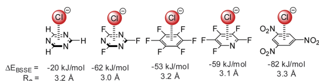
Fig. 2 Interaction energy with basis set superposition error correction ( E_{\text{BSSE}} ) and equilibrium distances ( R_e ) of selected anion- \pi complexes from the MP2/6-311++G** level of theory. 7,15,16
