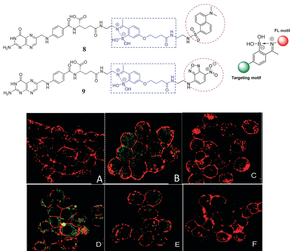
Fig. 11 Proposed structure of N-B based cancer cell targeting fluorescent conjugates 8 and 9 . Optical imaging of xenograft tumor by the specific boronate-fluorophore. (A) HEK and (B) NCI-H460 cells were incubated with compound 8 ; (C) NCI-H460 and (D) NCI-H460 without and (E) with pre-treatment with EDA-FA were incubated with compounds 9 ; (F) NCI-H460 treated with no boron compound. Images show an overlay of the emission of compounds in the 460–580 nm regions upon excitation at 458 nm (green), and the emission of the membrane marker in the 650–700 nm regions upon excitation at 514 nm (red). Reproduced with permission from ( Chem. Commun. , 2014, 50 , 5261). Copyright © 2014 Royal Society of Chemistry.
