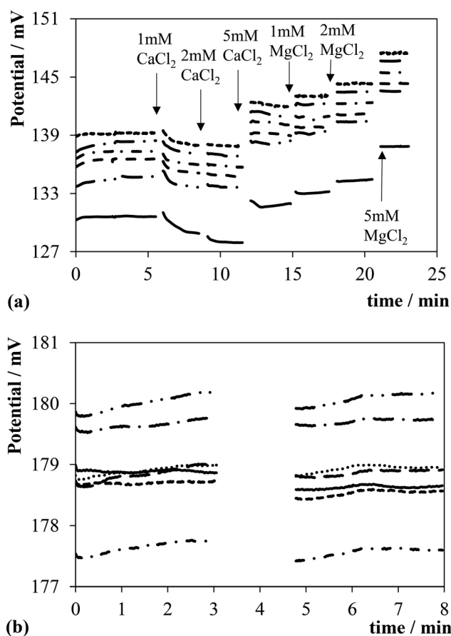
Fig. 2 Each line represents the individual trace of the \Delta E of six IrOx-coated needles immersed in a phosphate buffer ( \text{pH} = 6.80 \pm 0.05 ) containing (a) 0.1 M KCl or (b) 0.1 M \text{KNO}_3 . (a) The buffer was spiked with 0.4 M aqueous \text{CaCl}_2 and 0.4 M aqueous \text{MgCl}_2 at the time indicated by the arrows and the resulting concentrations of \text{CaCl}_2 and \text{MgCl}_2 are reported in the graph. (b) Albumin was added at t = 3 min in order to obtain a final concentration of 1 \text{ g L}^{-1} and after 2 minutes of stirring without recording the measurements were then re-started under quiescent conditions.
