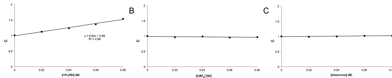
Fig. 2 Stern–Volmer quenching studies for (A) i -Pr 2 NEt, (B) LiBF 4 , and (C) enone 6 .
