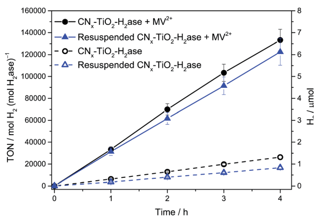
Fig. 3 Photocatalytic H 2 production using Dmb [NiFeSe]-H 2 ase (50 pmol) in EDTA (pH 6, 0.1 M, 3 mL) with CN x -TiO 2 (5 mg) under optimised conditions before and after centrifugation and re-suspension in fresh EDTA buffer solution followed by 1 Sun irradiation ( \lambda > 420 \text{ nm} ). Results are also shown in the presence and absence of redox mediator, methyl viologen (MV 2+ ).
