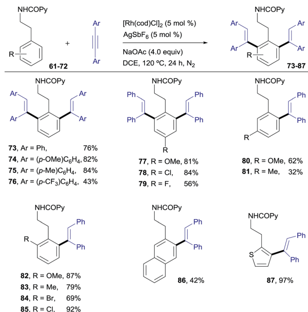
Scheme 6 Rh I -catalyzed ortho -olefination of phenethylamine derivatives.
