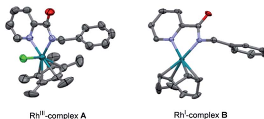
Fig. 2 ORTEP view of Rh III -complex A and Rh I -complex B. The hydrogen atoms have been removed for simplicity.
