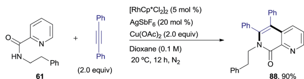
Scheme 7 Rh III -catalyzed pyridyl C–H functionalization leading to a 1,7-naphthyridin-8(7H)-one derivative.
