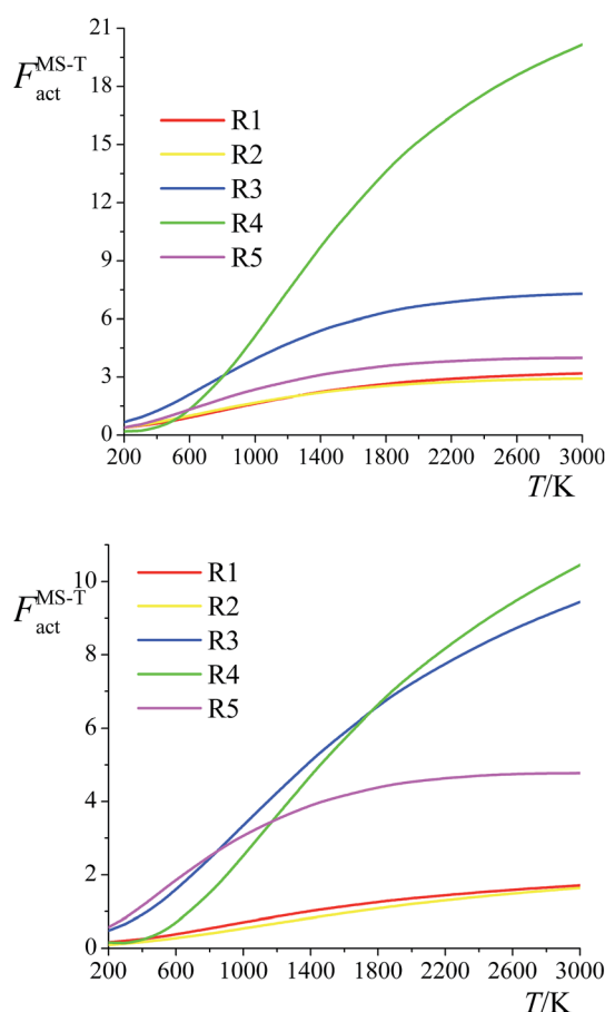
Fig. 6 Multistructural torsional anharmonicity factors F_{\text{act}}^{\text{MS-T}} for: (top) Forward reactions (R1)–(R5); (bottom) Reverse reactions (R1)–(R5).
