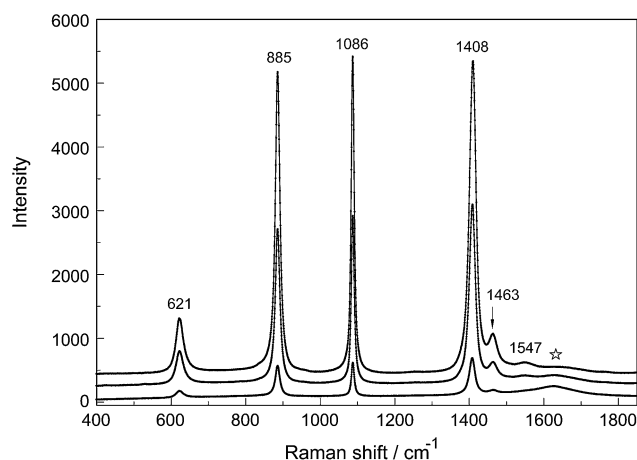
Fig. 8 Concentration profiles of the isotropic scattering of NaCD 3 CO 2 (aq): from top to bottom: (A) 2.936 mol L −1 , (B) 1.468 mol L −1 , (C) 0.294 mol L −1 . The open star denotes the scattering contribution of the deformation mode of water and the mode denoted by the arrow indicates the combination band at 1463 cm −1 . The bands at 1408 and 1547 cm −1 are due to the symmetric stretch of the –CO 2 group while the mode at 885 cm −1 are the stretching mode of C–C and the mode at 621 cm −1 is due to the rocking mode of the –CO 2 group. (The strong mode at 1086 cm −1 is due to the CD 3 deformation mode.)
