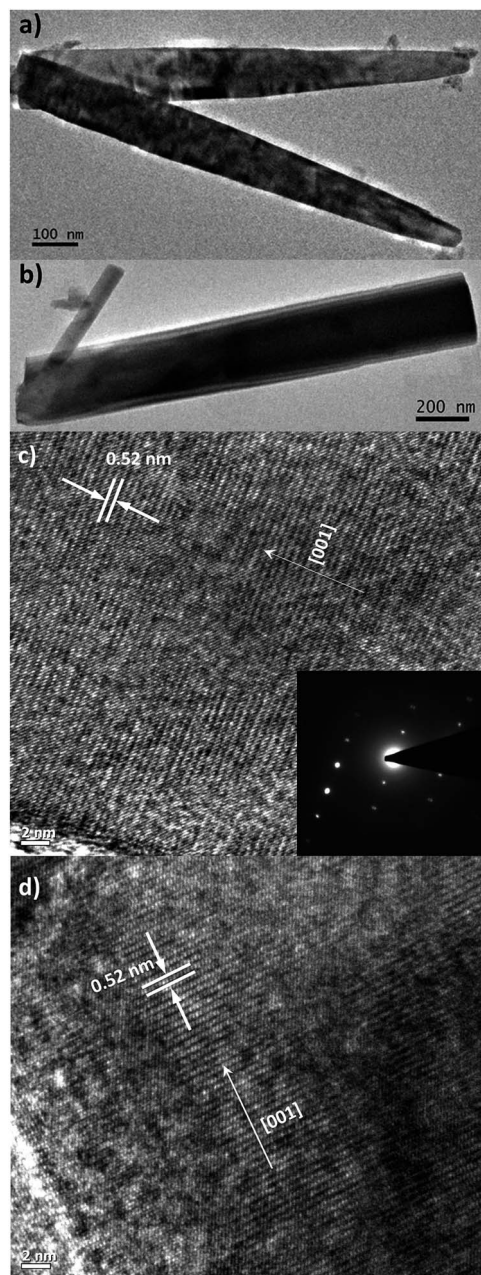
Fig. 2 Low-resolution TEM images of (a) ZnO/ITO and (b) ZnO/Zn nanorods. High-resolution TEM images of (c) ZnO/ITO and (d) ZnO/Zn nanorods. Inset shows the SAED pattern of ZnO/ITO nanorods.
