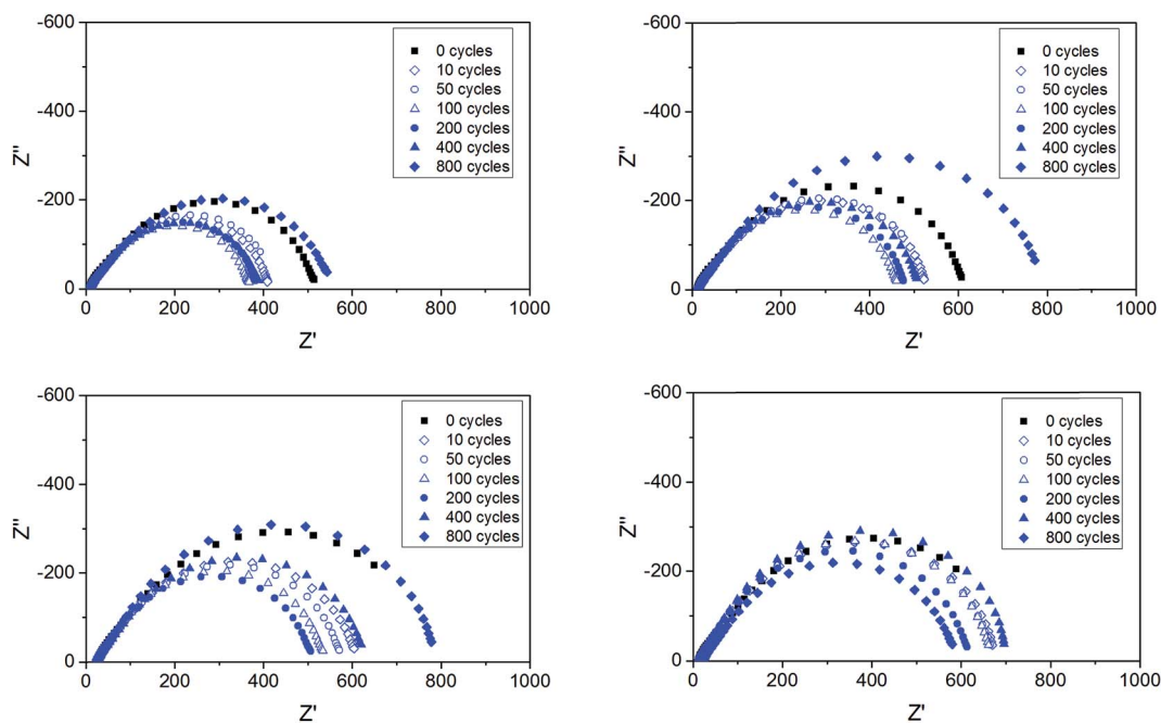
Fig. 10 Electrochemical impedance spectra of ternary electrolytes containing Pyr 14 TFSI (left, top) and Pyr 1201 TFSI (right, top), Pyr 14 BETI (left, bottom) and Pyr 1201 BETI (right, bottom) recorded at 21 °C during the plating–stripping cycle test at 40 °C. Frequency range: 100 kHz–1 Hz.
