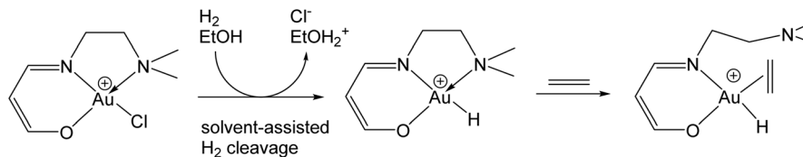
Scheme 7 Computational models for proposed intermediates in alkene hydrogenation catalysed by Au(III) Schiff base complexes. 50
