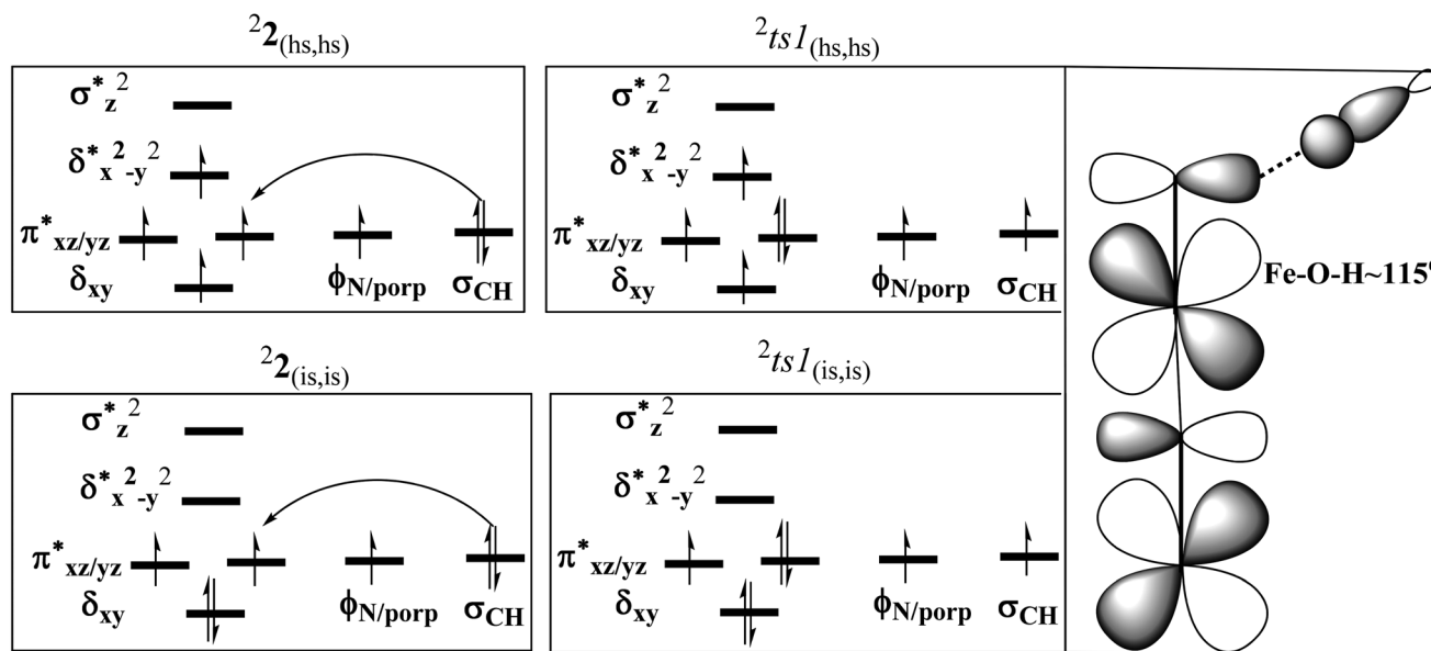
Fig. 6 The orbital evolution diagram for the C–H activation of 2^{2ts1(is, is)} and 2^{2ts1(hs, hs)} .
