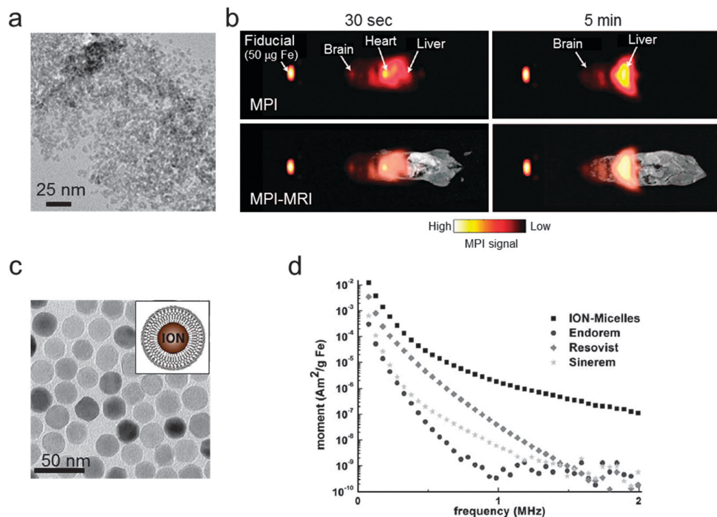
Fig. 8 MPI–MRI dual-mode imaging agents. (a) TEM image of Resovist ® . (b) Full-body MPI–MRI dual-modal imaging using Resovist ® for the in vivo biodistribution study. Resovist ® is observed in the brain, heart, and liver 30 sec after injection, followed by significant accumulation in the liver after 5 min. (c) TEM image and schematic illustration of ION-Micelles. (d) The MPI signal generating capabilities of the various iron oxide nanoparticles (ION-Micelles, Endorem ® , Resovist ® , and Sinerem ® ) as shown in the plot of the magnetic moment vs. the oscillating magnetic field frequency. The higher magnetic moment of ION-Micelles compared with the other nanoparticles over the entire frequency range allows for a stronger MPI signal. (a) Reprinted with permission from ref. 42. Copyright 2012, American Institute of Physics. (b) Reproduced from ref. 40 by permission of John Wiley & Sons Ltd. (c and d) Reproduced with permission from ref. 43. Copyright 2013 Starmans et al.
