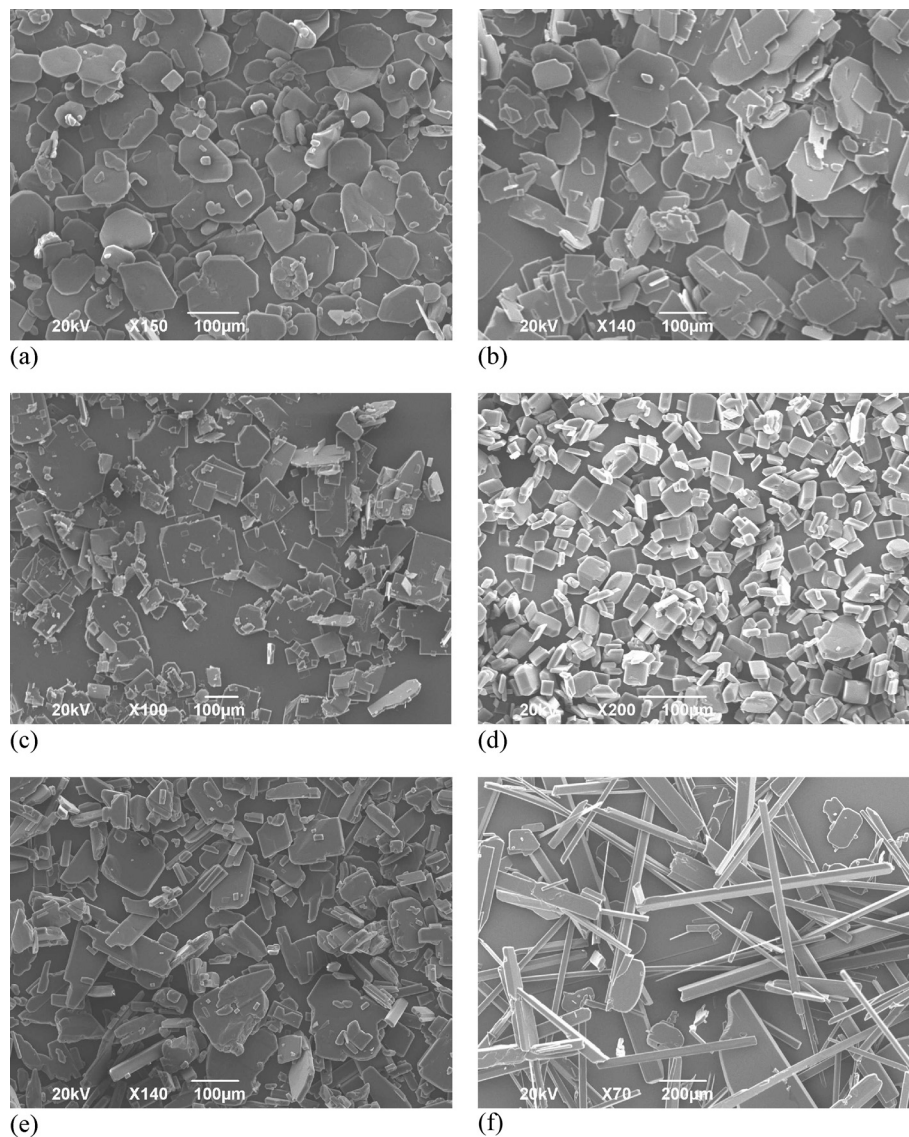
Fig. 10 FI recrystallized by cooling ( \Delta T = 5\text{ }^{\circ}\text{C} ) in (a) acetic acid, (b) acetone, (c) acetonitrile, (d) n -butanol, (e) toluene with agitation and (f) toluene without agitation.
