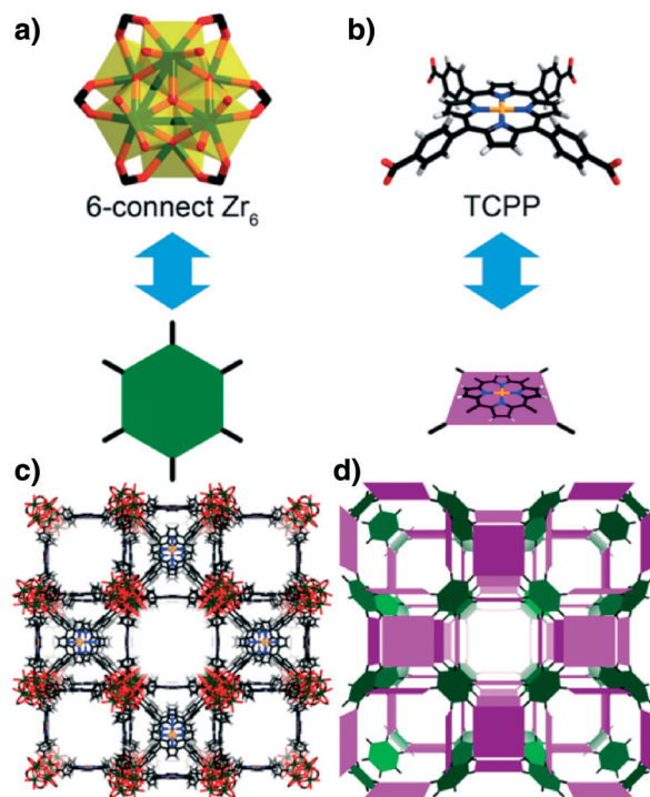
Fig. 4 The 6-connected D_{3d} symmetric Zr_6 (a) in PCN-224 and tetatopic TCPP ligands (b) with twisted dihedral angles generate a framework with 3D nanochannels (c, d). Colour scheme: Zr, green spheres; C, grey; O, red; N, blue; Ni, orange; and H, white. (Reproduced from ref. 24 with permission, Copyright 2013 American Chemical Society.)
